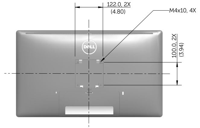
Back View of Monitor without stand
